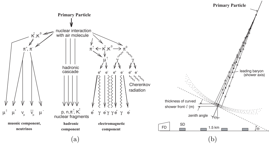
Figure 2.2.: In (a), the main processes taking place in extensive air showers are denoted. Specifically, the muonic, the hadron and the neutrino component as well as the electromagnetic component are indicated. In (b), the profile of a typical air shower is shown; the shower axis and the shower front are sketched in the figure. Taken from [Kei03].
