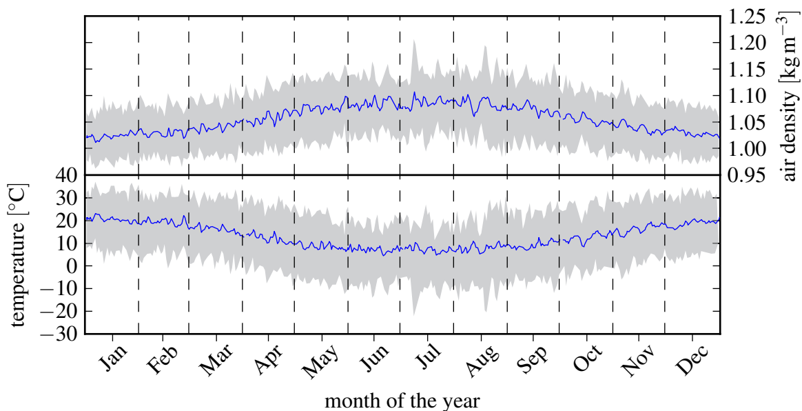
Figure 4.2.: Variation of the air density and temperature on a seasonal scale, averaged over a time period of 5.5 years (June 2004 to December 2009), at ground level of the CLF. Upper pane: Density of the air during the course of a year. Lower pane: Temperature of the air during the course of a year. The light grey areas depict the ranges that are covered by the quantities during the respective days of the year. The solid line results from a convolution of the instantaneous values with a (24 hours) top-hat window function. To avoid boundary effects, one day of data at the end of the time period has been prepended to the first day prior to convolution.
